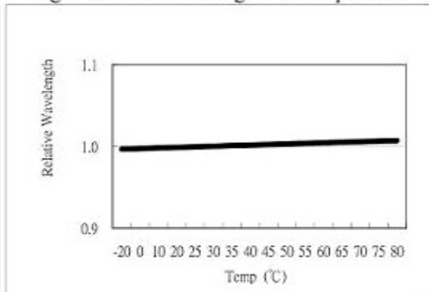
Fig4. Relative Wavelength vs. Temperature
